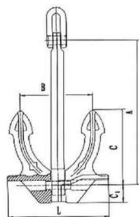
无杆锚 Stockless Anchor
